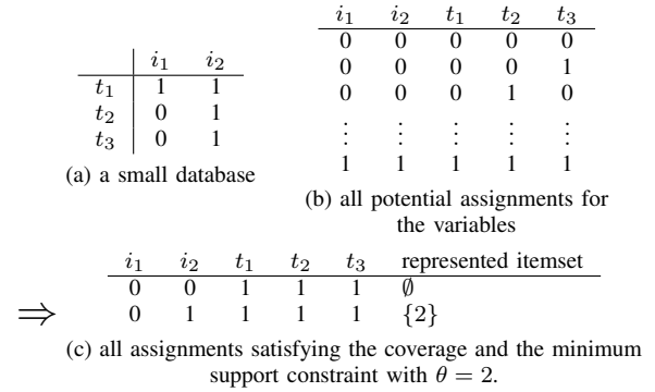
Fig. 1. Illustration of the potential solutions selected by a minimum support constraint for a given database.
